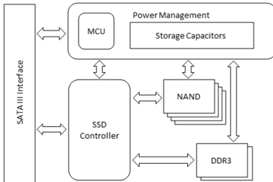
Figure 2-1: Block diagram for ATP SATAIII SSD
